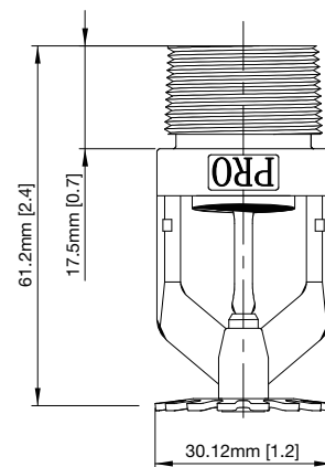
Pendent Sprinkler - PS304
