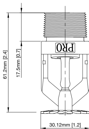
Pendent Sprinkler - PS302
