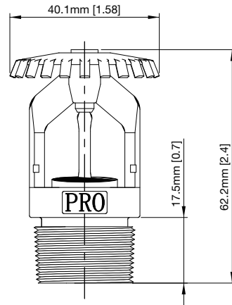
Upright Sprinkler - PS305
