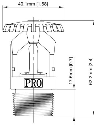
Upright Sprinkler - PS301
